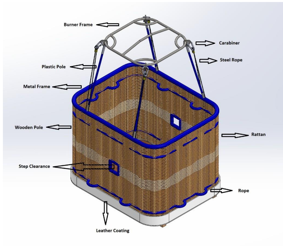
Figure 22. Basket general view
